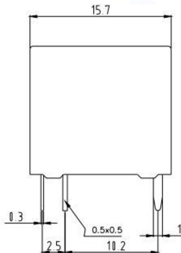
Outline Dimension
